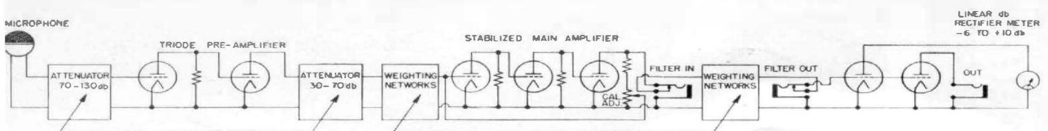
Figure 2. Elementary Schematic (or Functional diagram) Type 1551-A Sound-Level Meter.
