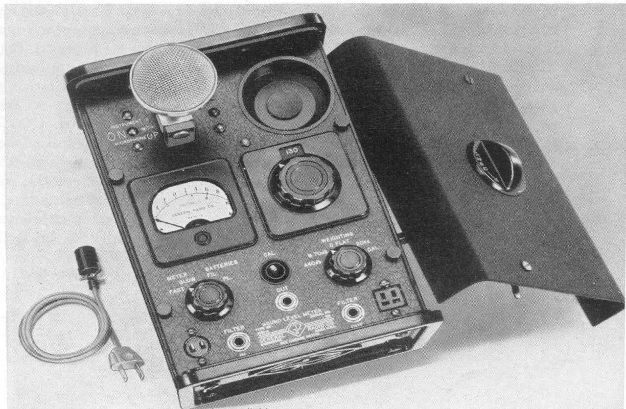
Figure 1. Panel View Type 1551-A Sound-Level Meter.
