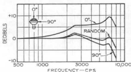
Figure 7. (Right) Typical acoustic and electrical calibration curves for the Type 1551-A Sound-Level Meter.
