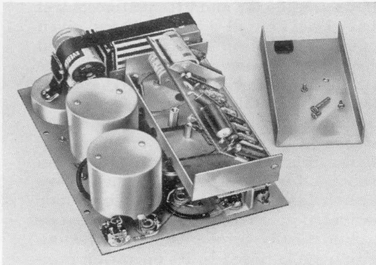
Figure 3. View of Type 1551-A removed from its case. Amplifier cover removed, and amplifier raised to show accessibility.
