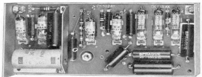
Figure 4. Detail view of panel side and bottom side of Amplifier Shelf.
