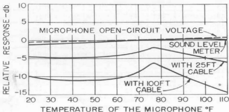
Figure 8. Variation in response as a function of temperature for the microphone alone and with various lengths of cable between microphone and sound-level meter.
