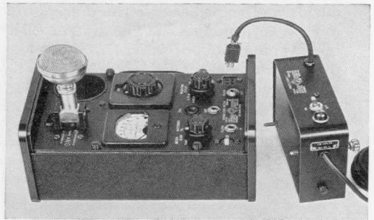
Figure 5. Type 1551-A with Type 1262-A A-C Power Supply.
